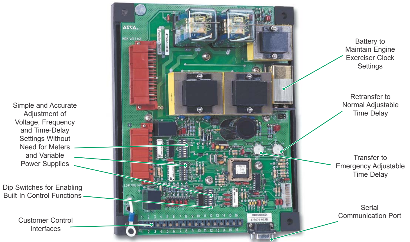
Fig. 9: Microprocessor Controller
